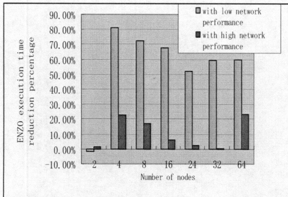
Figure 8. Comparison of ENZO Execution Time Reduction under Different Networking Performance
