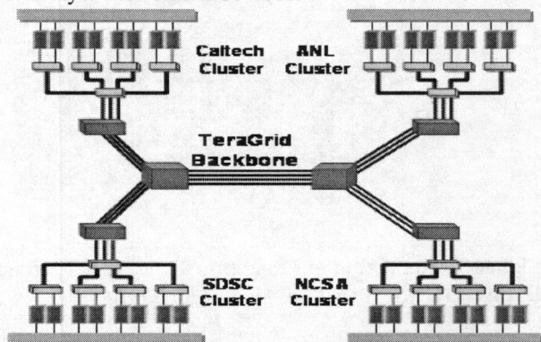
Figure 3. Network architecture of TeraGrid
