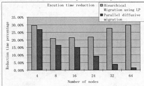
Figure 7. Reduction of Execution Time with Synthetic Datasets (DistPM vs. Diffusive Algorithm)
