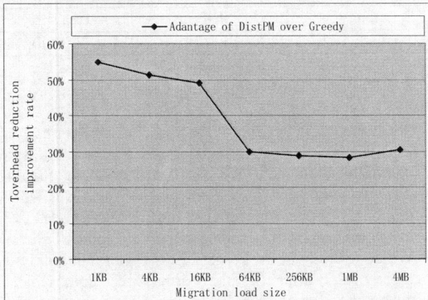
Figure 4. Reduction of Communication Cost with Synthetic Datasets (DistPM vs. Greedy Algorithm).
