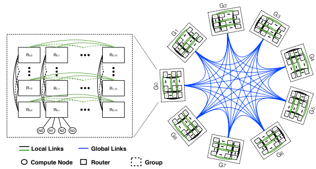
Fig. 1: Overview of the dragonfly system configuration
