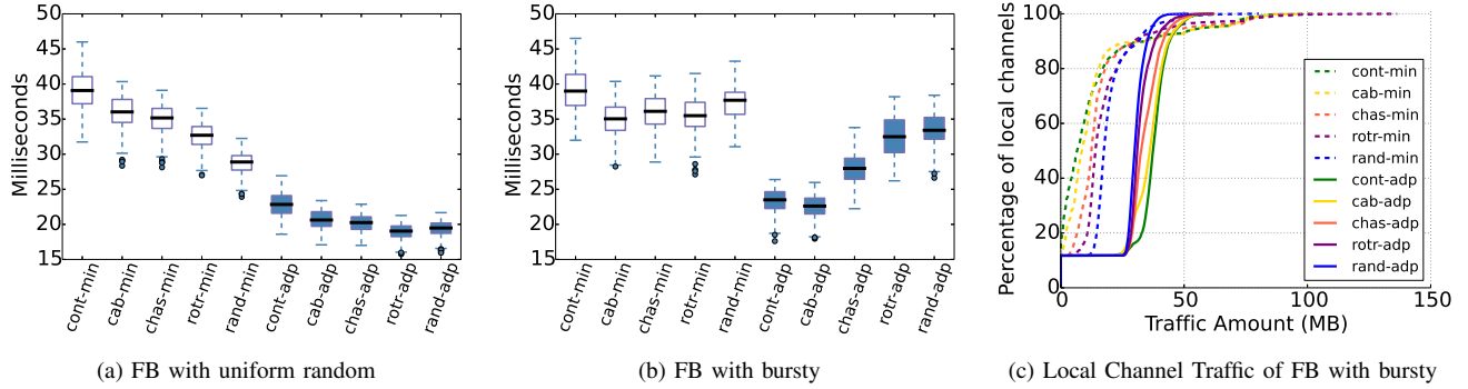
Fig. 10: Communication time and local channel traffic of FB with background traffic.
